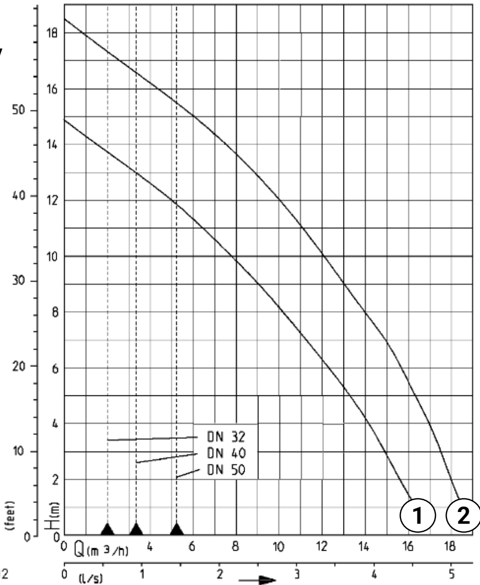
Multicut 08/2MES 230V Pumpkurva 1
